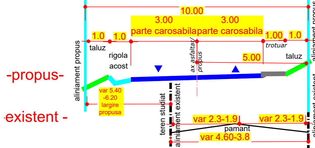
PROFIL TRANSVERSAL CARACTERISTIC e-e scara 1:100
