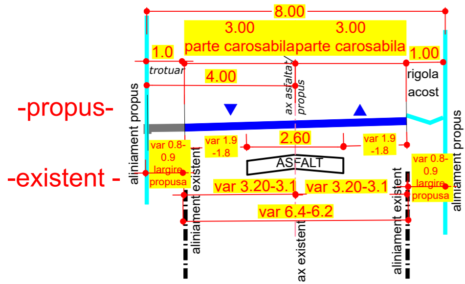
PROFIL TRANSVERSAL CARACTERISTIC -a-a scara 1:100
